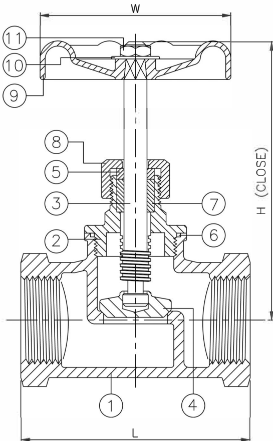
Figure # 41276 = 200#, 316, NPT, Globe Valve
